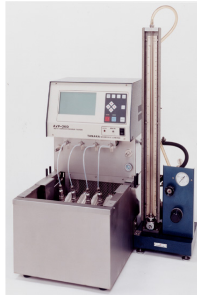
AVP-30D-4bombs & Mercury Manometer
